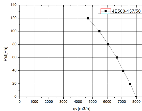
FLOW RATE CURVE (风量曲线) :
